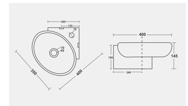
► NEW CORNER 350x400x145mm
