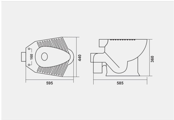
▶ HARNI -3009 P-Trap 595x440x360mm Anglo Indian E.W.C.
