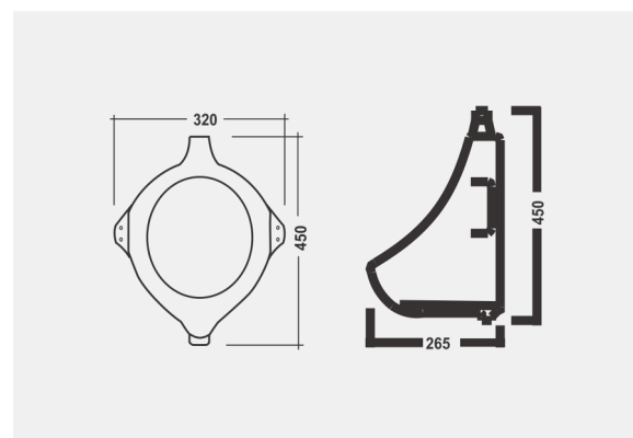
► FLAT BACK URINAL 320x265x450mm
