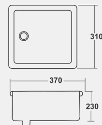
► KITCHEN SINK 370x310x230mm (12"x10"x7")
