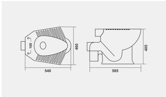
▶ HARNI -3009 S-Trap 540x460x405mm Anglo Indian E.W.C.
